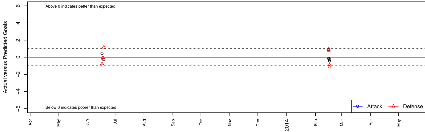
Colorado Storm Copa B97 Dots are actual minus expected GF (blue circles) and GA (red triangles). Blue line is smoothed change in attack strength. Red is smoothed change in defense strength.
